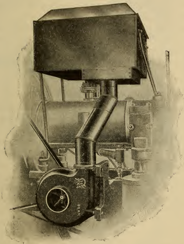
FIG. 62.—WATER-COOLING DEVICE OF THE "OTTO" GASOLINE TRACTION ENGINE.
